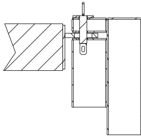
Single-Lockbox SECTION A-A SCALE 1 / 16
