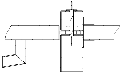
Single lock SECTION L-L SCALE 1 / 16
