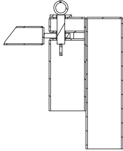
Single lock SECTION G-G SCALE 1 / 16
